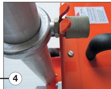
Mounting the mast on the battery/charger case is secured with a single thumb screw.
