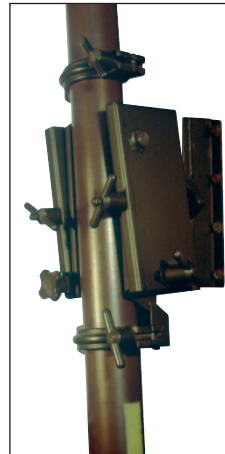
SHELTER OR VEHICLE MOUNTING Cat. No. 10481
